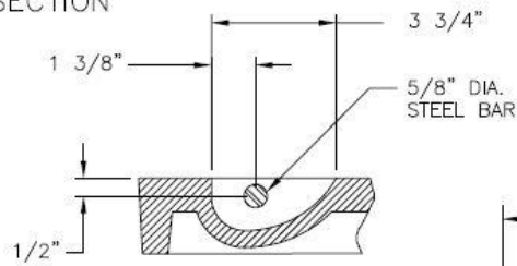
COVER SECTION
