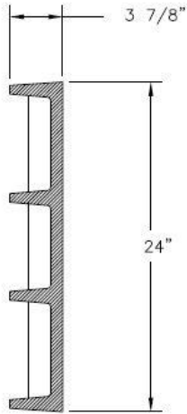
COVER SECTION
